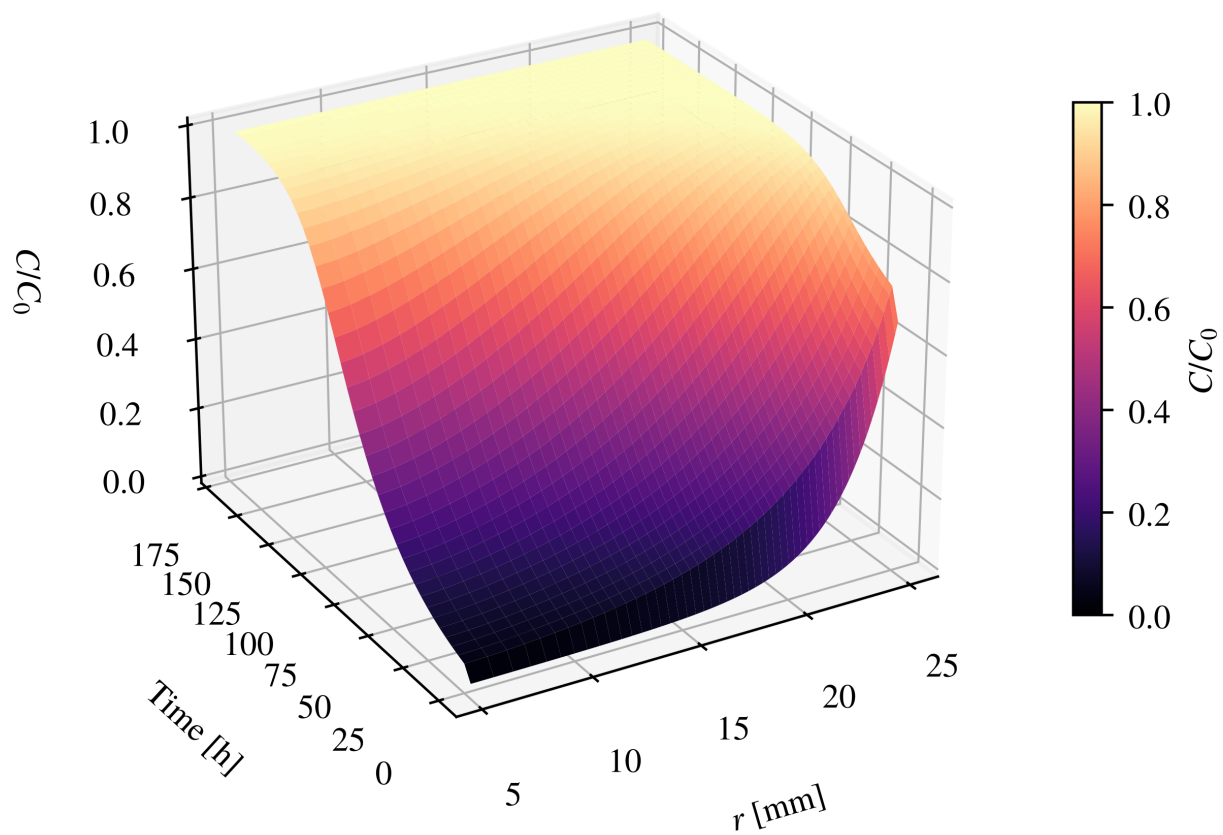
Figure 3. Three-dimensional view of the concentration field C(r, t)/C_0 .
