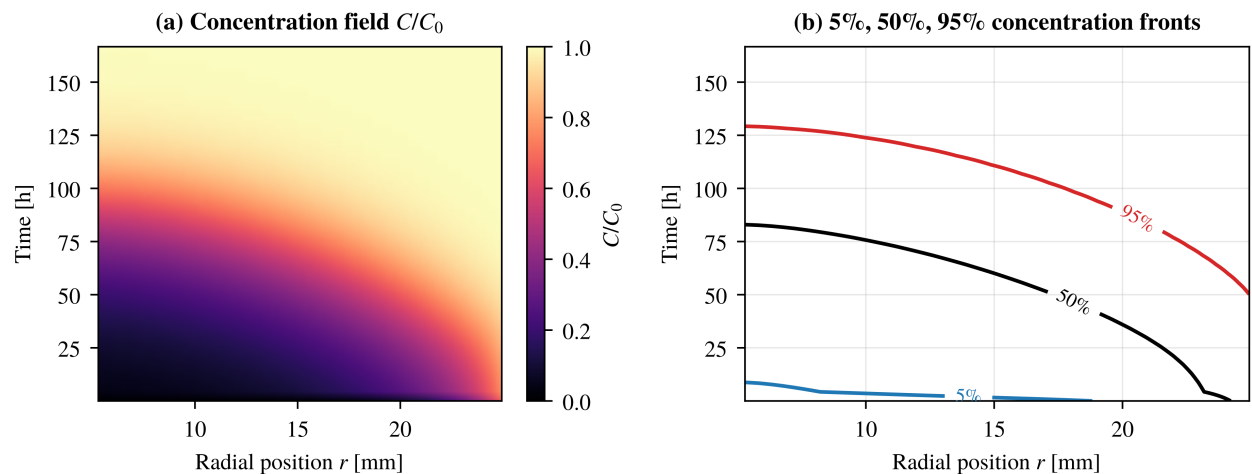
Figure 2. Space–time evolution of C/C_0 : (a) field map; (b) 5%, 50%, and 95% concentration fronts. The front reaches the core (outlet) later than the outer surface (inlet).
