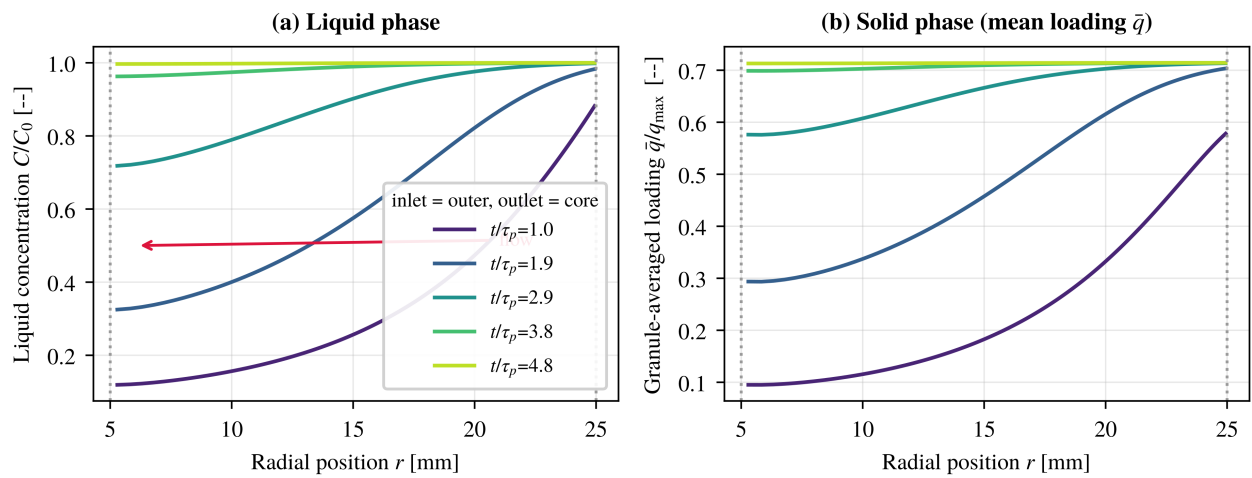
Figure 1. Radial profiles at t/\tau_p = 1.0, 1.9, 2.9, 3.8, 4.8 : (a) liquid concentration C/C_0 ; (b) granule-averaged loading \bar{q}/q_{\max} . Flow is inward, from the outer inlet ( r = R_{out} = 25 mm) to the core outlet ( r = R_{in} = 5 mm).
