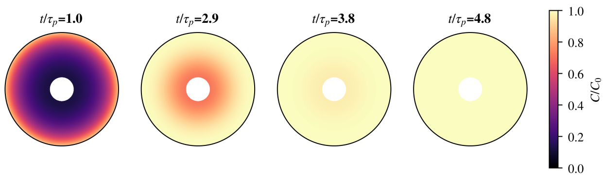
Figure 4. Annular cross-section (top view) of C/C_0 at t/\tau_p = 1.0, 2.9, 3.8, 4.8 ; the central hole is the perforated core (outlet). The saturation front propagates radially inward.
