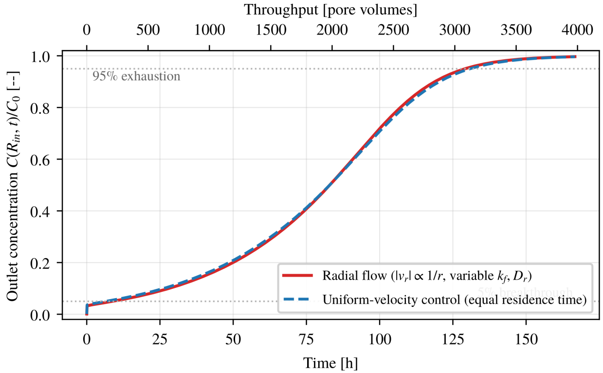
Figure 5. Breakthrough curve at the core outlet for the radial-flow filter (variable k_f , D_r ) and for a uniform-velocity control bed of equal residence time. Top axis: throughput in pore volumes.
