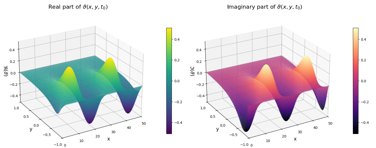
Figure 4. Real and imaginary parts of the transverse velocity component \vartheta(x, y, t_0) at t_0 = 25 , computed over the domains x \in [0, 50] and y \in [-1, 1] .
