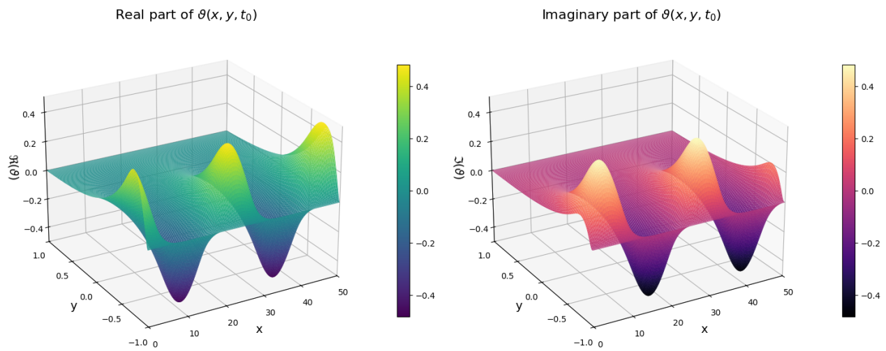
Figure 3. Real and imaginary parts of the transverse velocity component \vartheta(x, y, t_0) at t_0 = 0 , computed over the domains x \in [0, 50] and y \in [-1, 1] .
