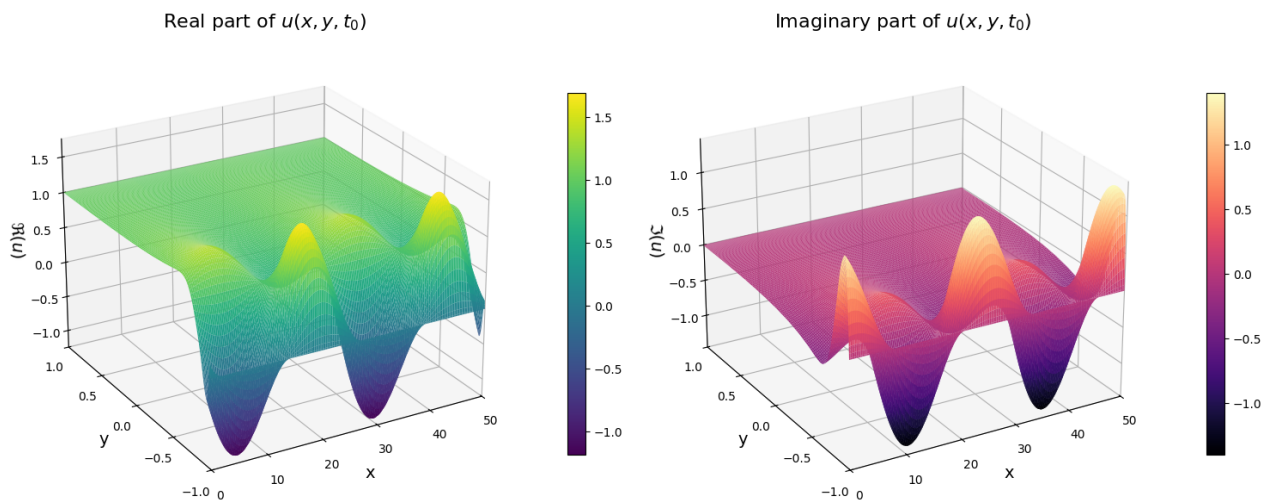
Figure 1. Real and imaginary parts of the streamwise velocity component u(x, y, t_0) at t_0 = 0 , computed over the domains x \in [0, 50] and y \in [-1, 1] .
