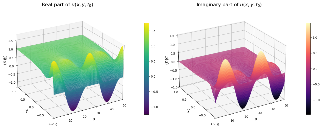
Figure 2. Real and imaginary parts of the streamwise velocity component u(x, y, t_0) at t_0 = 25 , computed over the domains x \in [0, 50] and y \in [-1, 1] .
