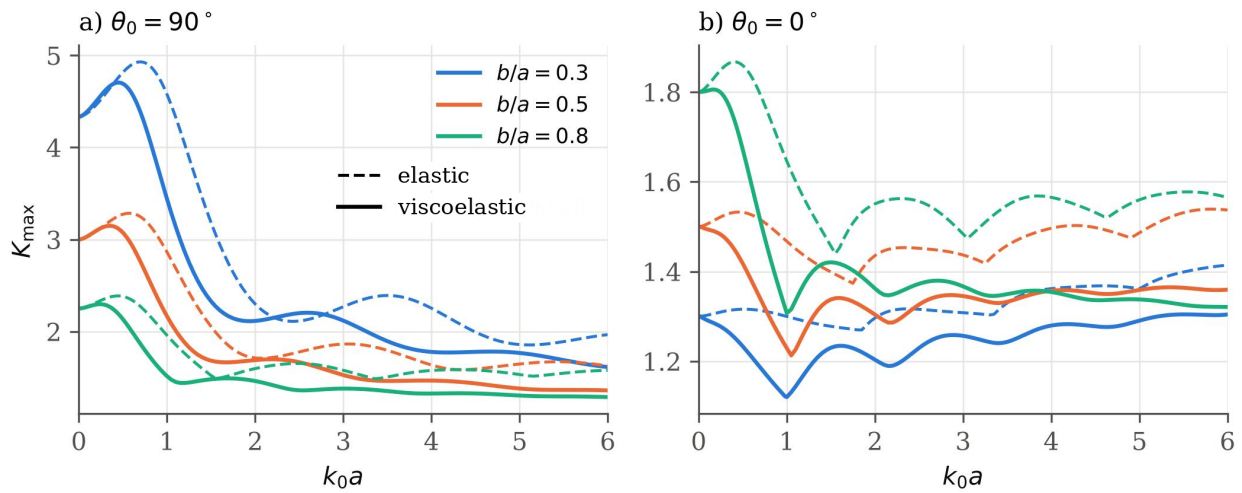
Figure 2. K_{\max} as a function of k_0 a : a) \theta_0 = 90^\circ (the wave is incident along the minor axis); b) \theta_0 = 0 (the wave is incident along the major axis). Dashed lines: elastic medium; solid lines: viscoelastic medium
