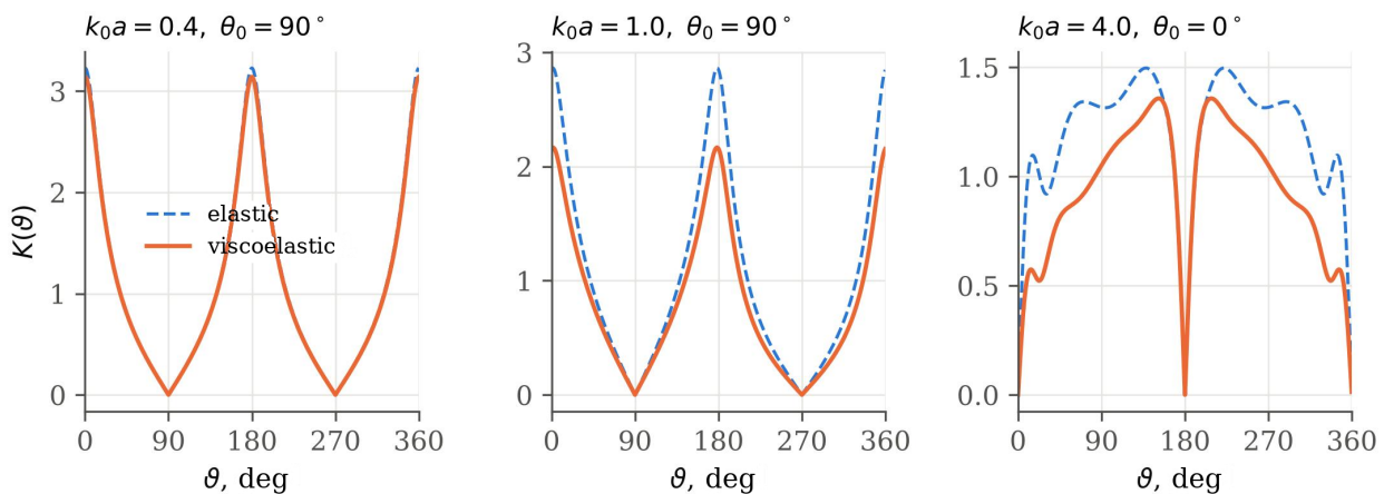
Figure 5. Distribution of the DSCF along the contour ( b/a = 0.5 ). Dashed line: elastic medium; solid line: viscoelastic medium
