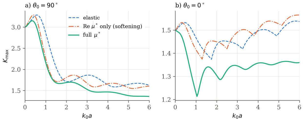
Figure 3. Separating the effect of viscosity ( b/a = 0.5 ): dashed line, elastic medium; dash-dotted line, modulus reduction only ( Re\mu^* ); solid line, full complex modulus
