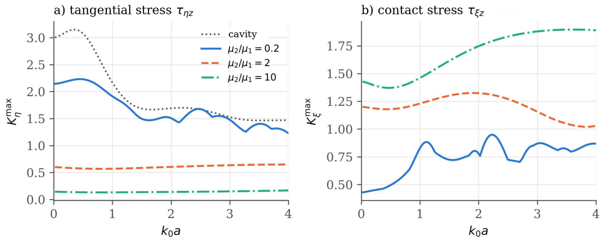
Figure 6. Effect of the filler stiffness ( b/a = 0.5 ; \theta_0 = 90^\circ ; both materials viscoelastic): a) tangential stress K_\eta ; b) contact stress K_\xi
