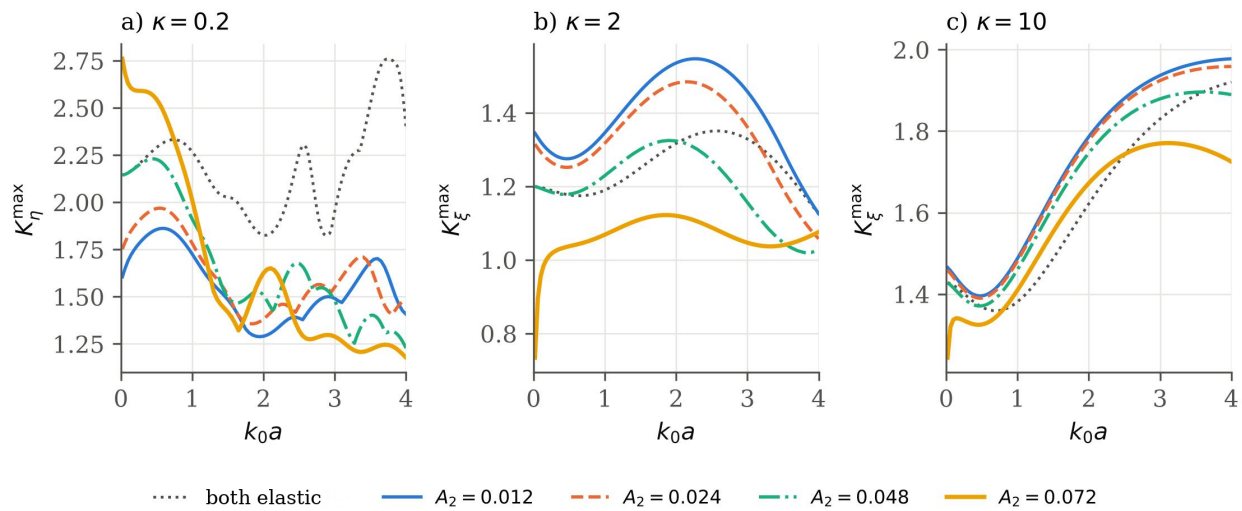
Figure 7. Effect of the filler viscosity ( A_2 ), A_1 = 0.048 ( b/a = 0.5 ; \theta_0 = 90^\circ ): a) soft filler, tangential stress; b), c) stiff filler, contact stress
