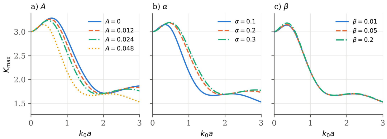
Figure 4. K_{\max} as a function of the kernel parameters ( b/a = 0.5 ; \theta_0 = 90^\circ ): a) A ( \alpha = 0.1 ; \beta = 0.05 ); b) \alpha ( A = 0.048 ; \beta = 0.05 ); c) \beta ( A = 0.048 ; \alpha = 0.1 )
